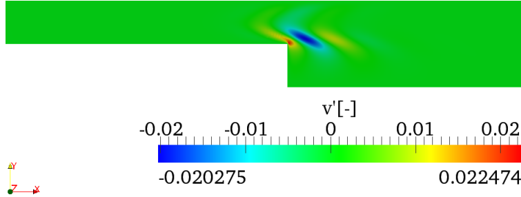
Figure 7: v' -component of the eigenmode
