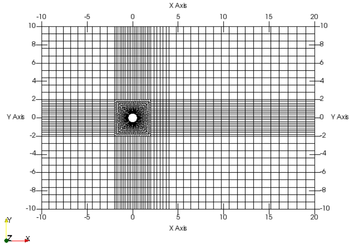
Figure 1.1 639 elements mesh.
